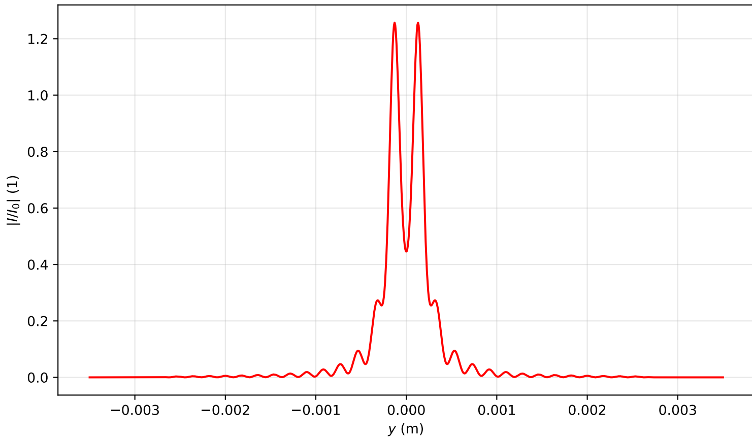
Intensity profile I(x=0, y, z=0.159)/I_0 , \text{Pin}=5.0\text{Pcr} , artificial time
